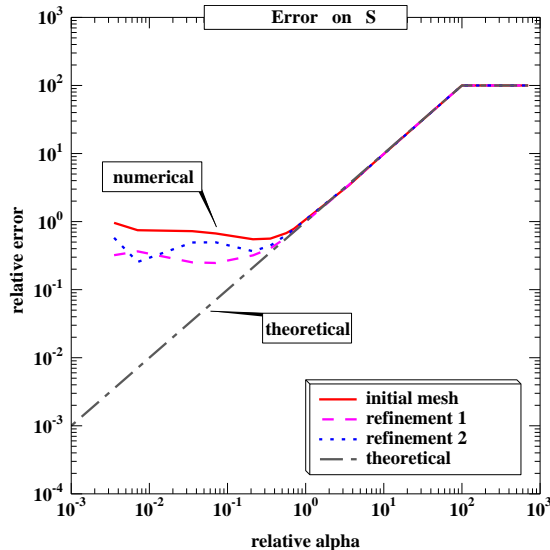
FIG. 3. Comparison between the theoretical and numerical errors.
