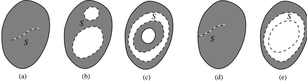
FIG. 2. In all cases \Gamma_0 is the whole boundary. The curve S is represented with a dashed line. In (a), (b) and (c) the geometrical hypothesis (1.4) is satisfied but not in (d) and (e). The set S_{ext} is shaded in each case.
