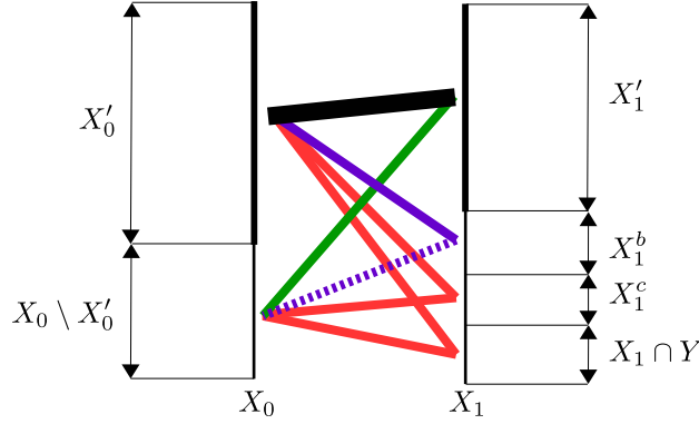
Figure 5.2: The terms in (5.15). The edges in the term e(X_0, (Y \cap X_1) \cup X_1^c) are shown in red, some edges of the term \sum_{u \in X_0 \setminus X'_0} h_0(u) are shown in green (note that we undercount here, as the summands h_0(u) reflect preliminary situations in the set X'_1 ). It is clear that each edge between X_1^b and X'_0 (solid blue) is counted in \sum_{v \in X_1^b} g_1(v) . Consider now an edge xv , x \in X_0 \setminus X'_0 , v \in X_1^b (dashed blue). Suppose first that x was removed from X'_0 before v was put in X_1^b . Then the edge xv was counted in \sum_{u \in X_0 \setminus X'_0} h_0(u) . Suppose next that v was put in X_1^b before x was removed from X'_0 . Then xv was counted in \sum_{v \in X_1^b} g_1(v) .
