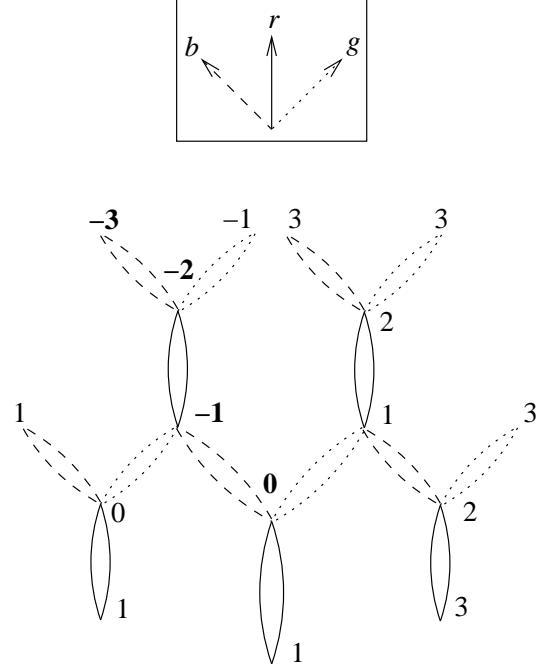
Figure 2: The Cayley tree \Gamma(G) for the three-color tiling, and the height function z .
