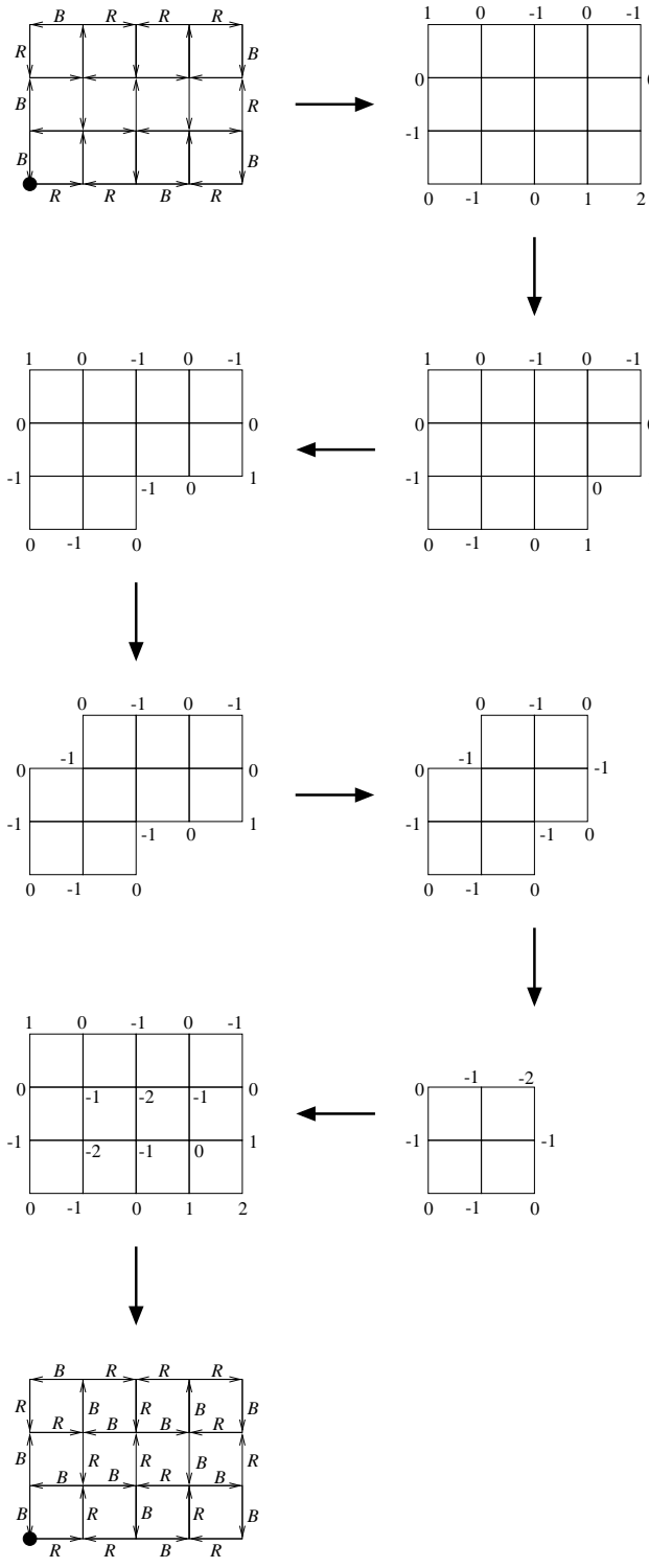
Figure 1: The progress of the tiling algorithm for W_{34} , or equivalently Eulerian orientations of the grid, which constructs the minimal tiling or shows that none exists.
