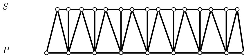
Fig. 5. A 2-connected interval graph with OD(G) \geq \frac{3}{2} \text{diam}(G) .
