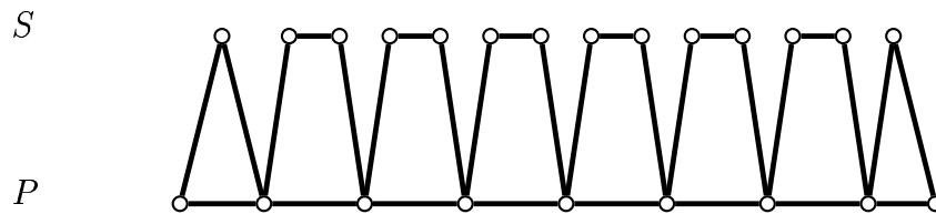
Fig. 1. A cocomparability graph with OD(G) \geq 2 \text{diam}(G) - 1 .
