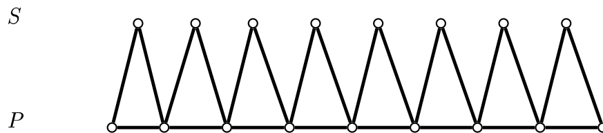
Fig. 2. A proper interval graph with OD(G) \geq \frac{3}{2} \text{diam}(G) .
