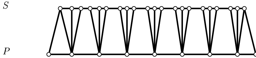
Fig. 4. A 2-connected cocomparability graph with OD(G) \geq 2 \text{diam}(G) - 1 .
