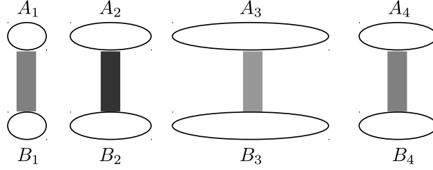
Figure 4.1: An example of an (\varepsilon, d, \ell) -regularized matching. Regular pairs are shown with a shade of grey corresponding to their densities.
