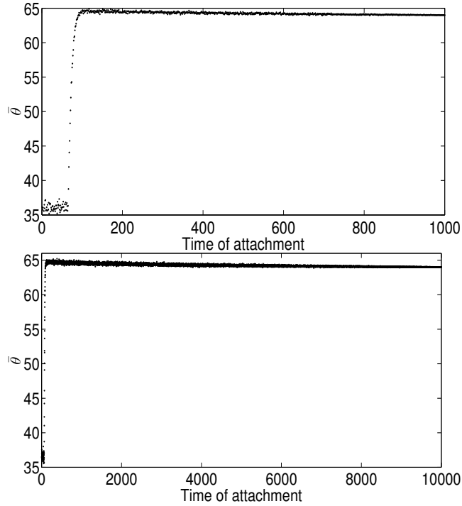
Figure 2: Values of \bar{\theta} . Top: N = 1000 and m = 64 . Bottom: N = 10000 and m = 64 .
